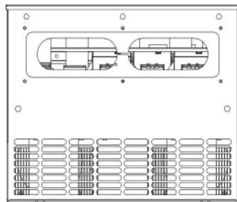
Dimensional drawing V810 - 160kW 4T1600
