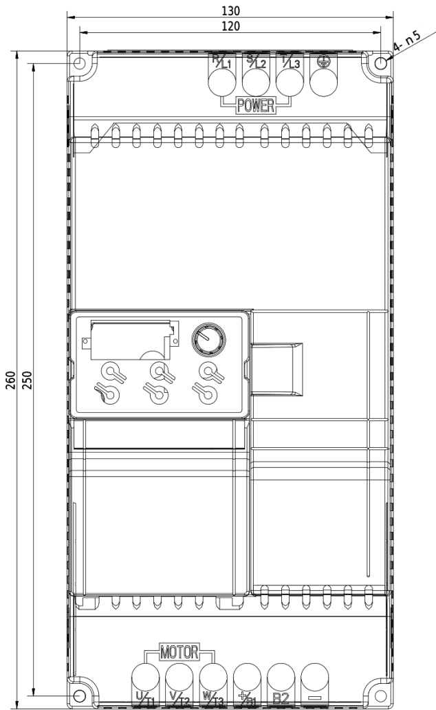
Dimensional drawing V800 - 7,5kW 4T0075
