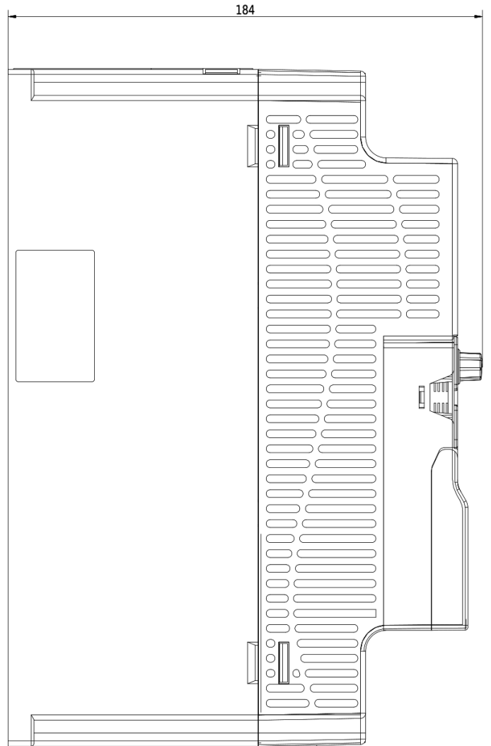
Dimensional drawing V800 - 11kW 4T0110
