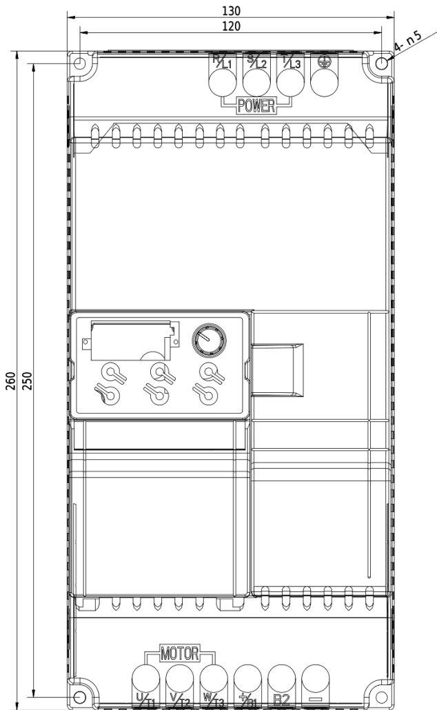
Dimensional drawing V800 - 11kW 4T0110
