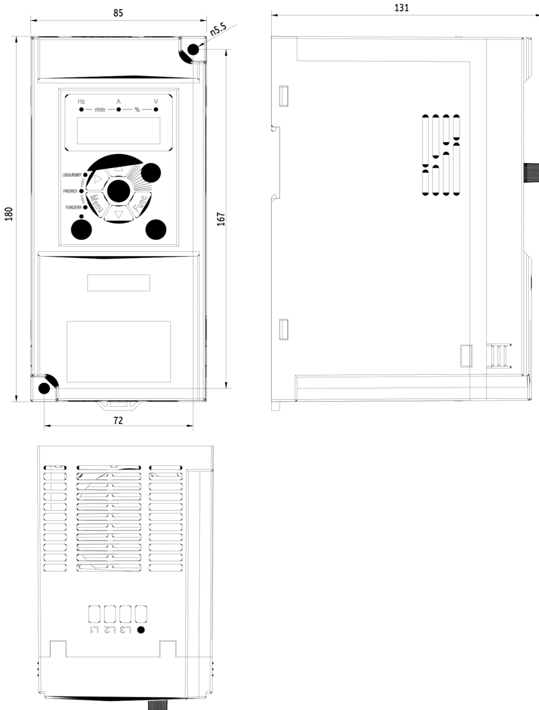
Dimensional drawing V900 - 7,5kW 4T0075
